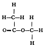
METHYL ACETATE.
